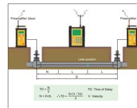
• Leak Correlating Loggers ZCORR
