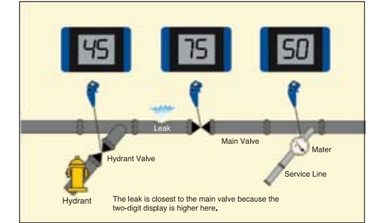
• Fuji Electric Listening Stick FSB-8D & Sound Judge FSJ-1
